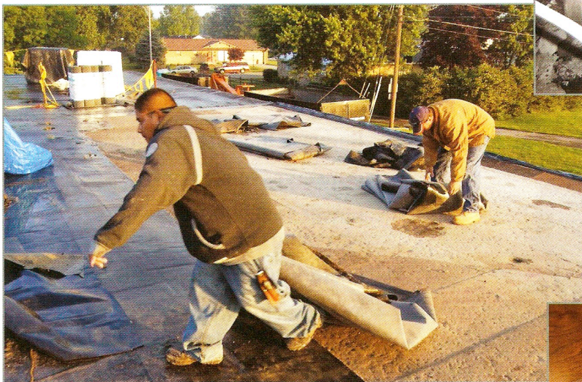
Photos 1, 2, and 3 – EPDM is removed from a ballasted system (above, left). Afterward, it is taken to the grinder (top right), and the final product results (bottom right). (Photos courtesy of ERA.)
