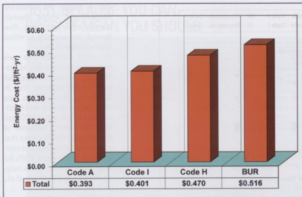
Figure 3 – Energy-cost savings is based on R-5 roof insulation and initial membrane reflectivity with HVAC rooftop air conditioner having seasonal COP of 2.5 (Miller et al., 2002).
