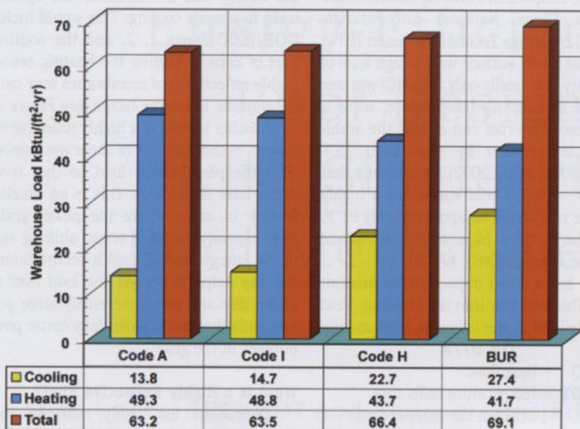
a. Annual building loads for warehouse.
